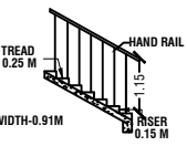
STAIRCASE DETAILS
