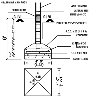
FOUNDATION DETAIL
