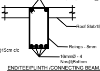
END/TEE/PLINTH/CONNECTING BEAM
