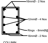
COLUMN
