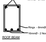
ROOF BEAM
