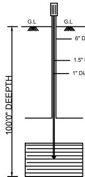
BORE WELL
