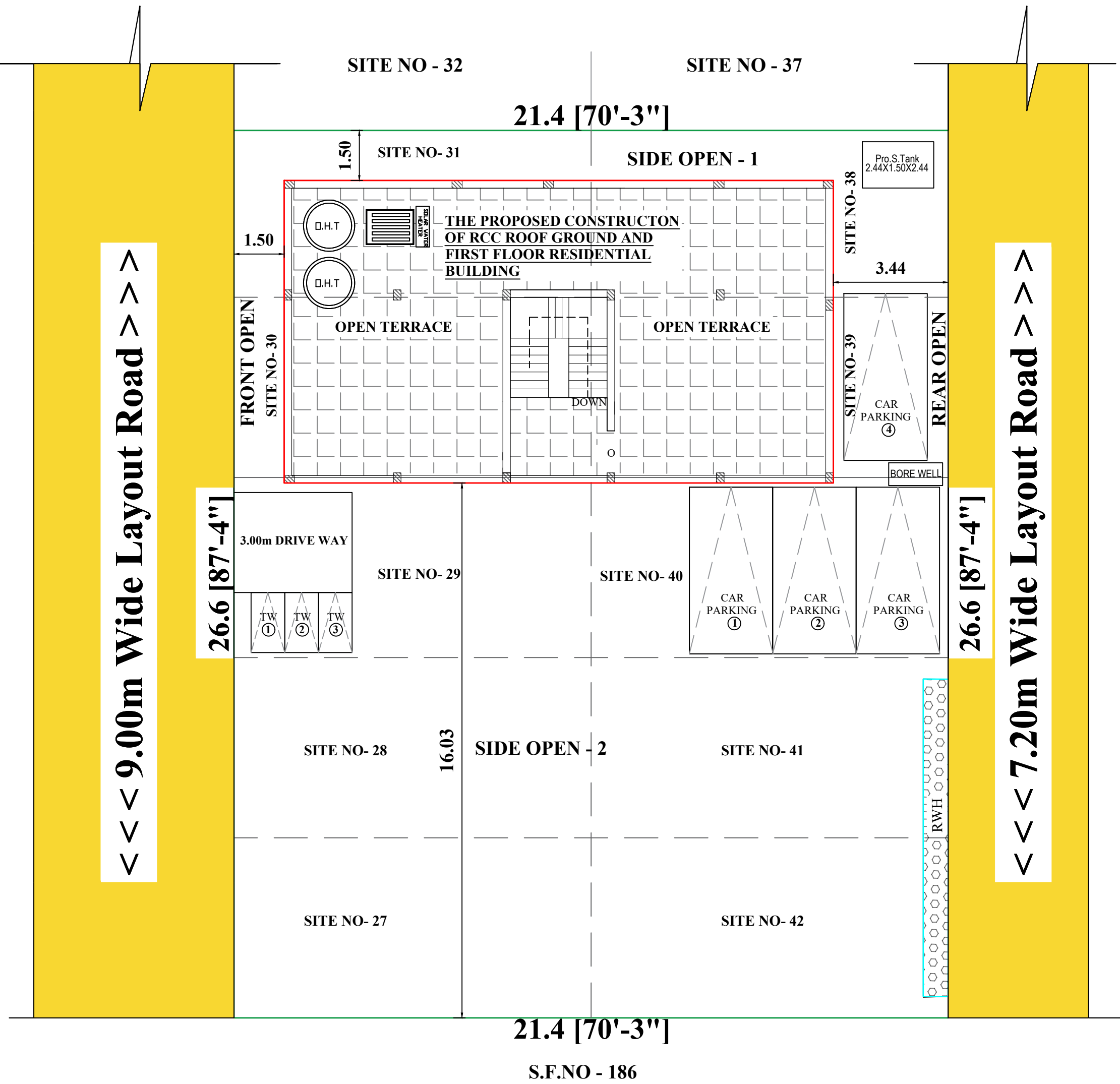
SITE PLAN & TERRACE PLAN
