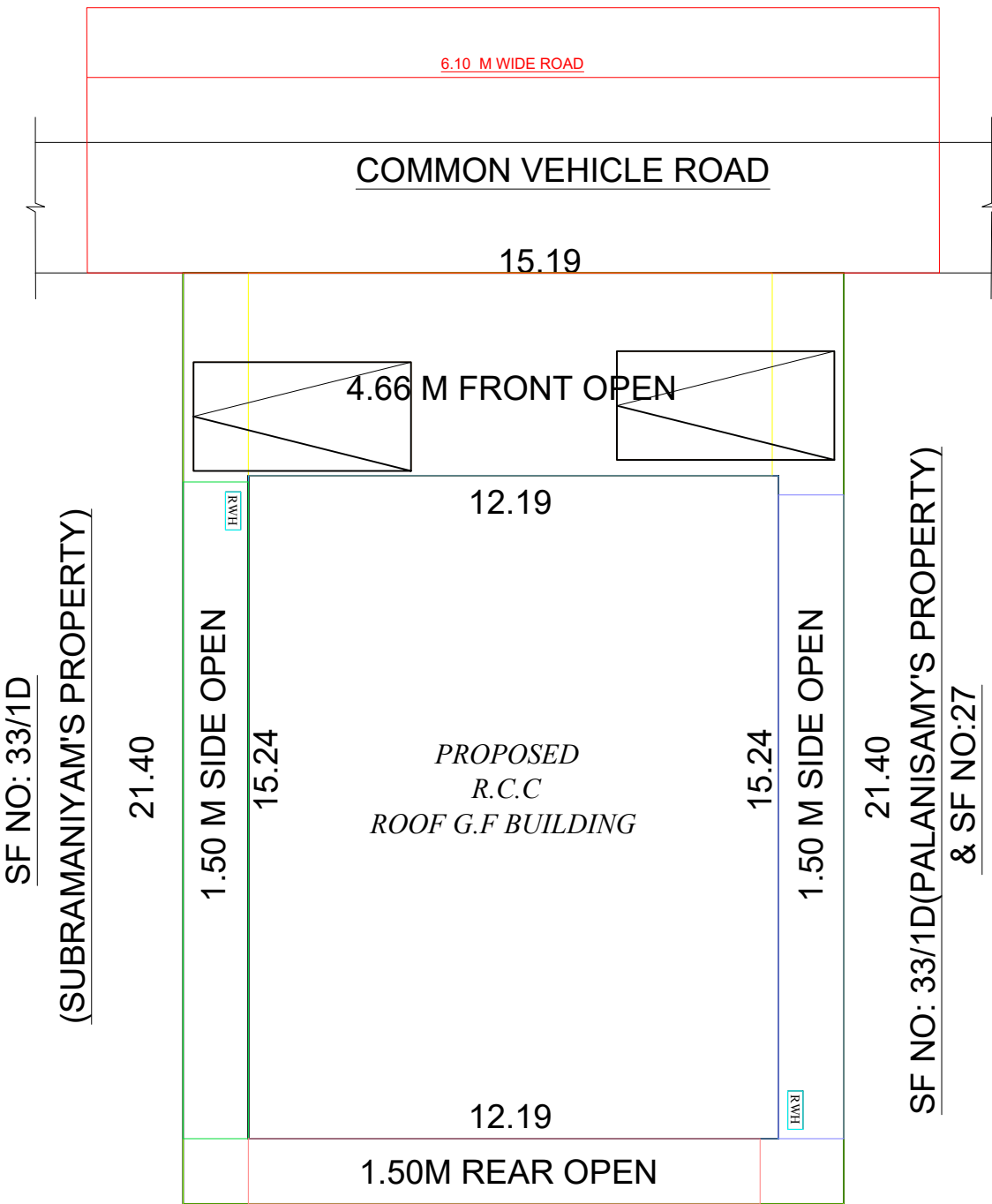
SF NO: 33/1D (SUBRAMANIYAM'S PROPERTY) SF NO: 33/1D(PALANISAMY'S PROPERTY) & SF NO:27 15.19 SF NO: 33/1E SITE PLAN (SCALE 1:100)
