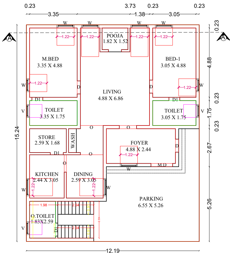
PRO. GROUND FLOOR (G.F) PLAN
