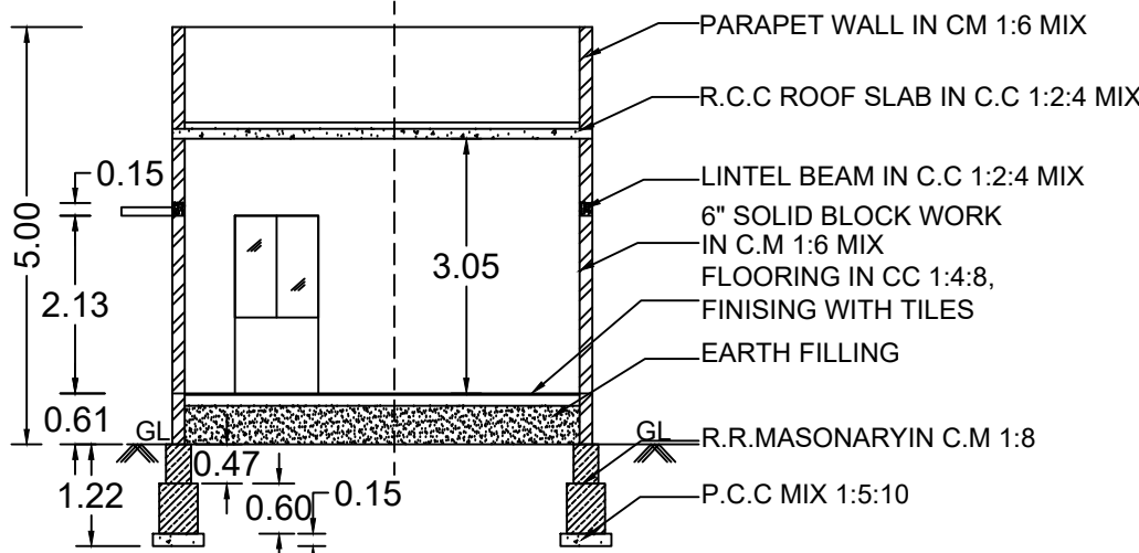
SECTION "A-B"
