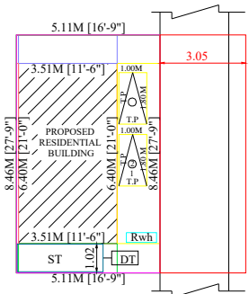
SITE PLAN(MEANT FOR CONSTRUCTION) →N
