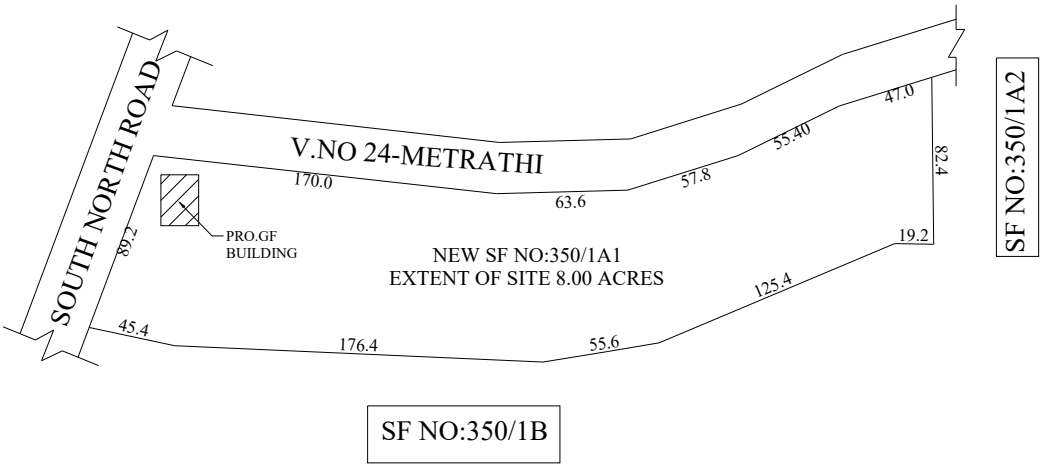
SITE PLAN(NTS)
