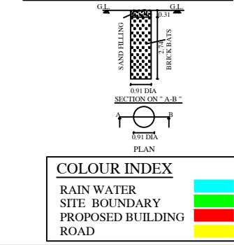
DETAILED PLAN OF RAINWATER PERCOLATION&COLLECTION PIT
