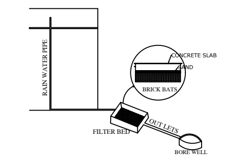
RAIN WATER HARVESTING TANK
