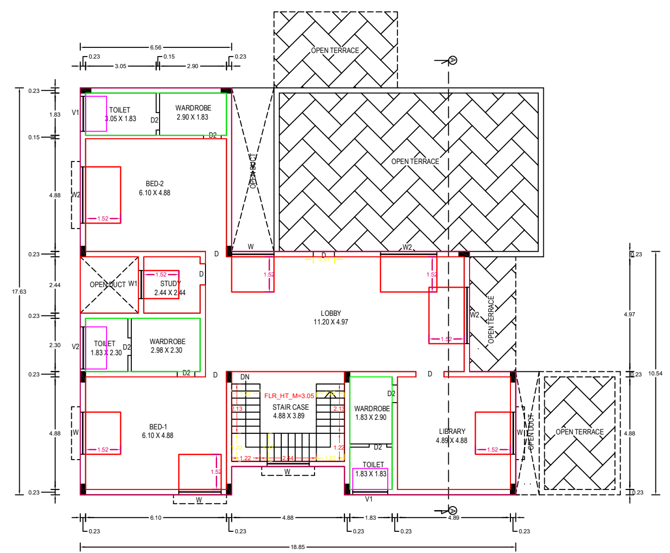
PRO. FIRST FLOOR PLAN.
