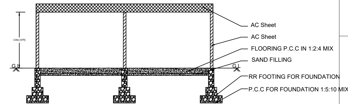
SECTION ON-AA
