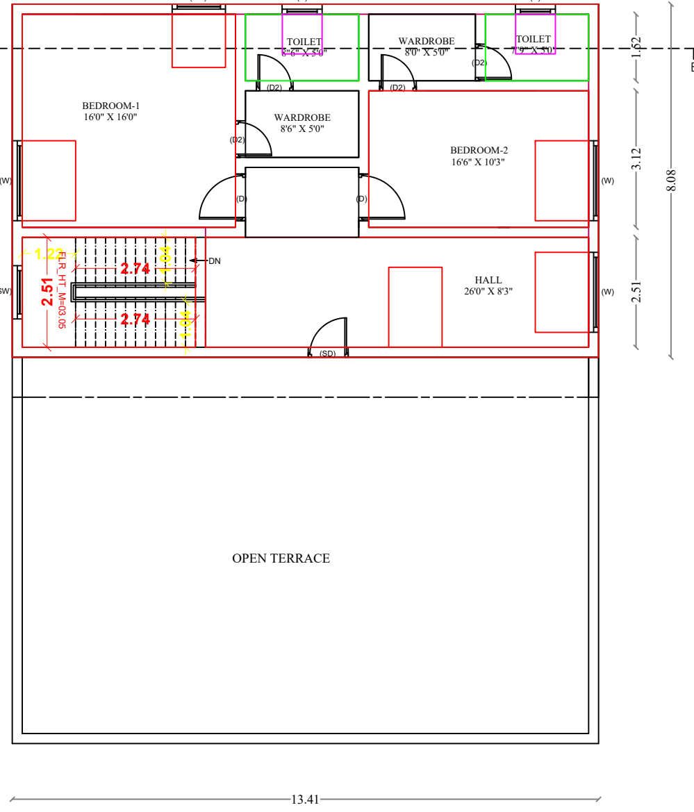
FLOOR-FIRST
