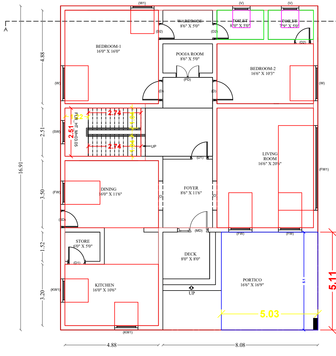
FLOOR-GROUND
