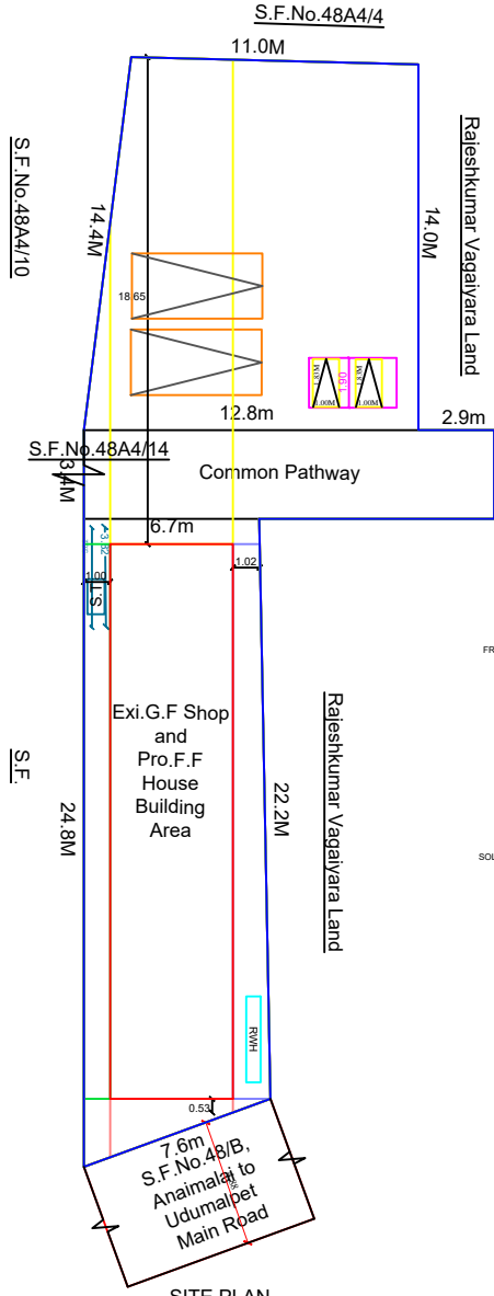
SITE PLAN
