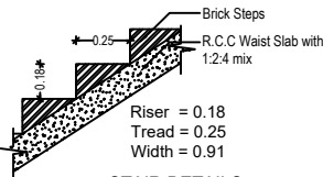
STAIR DETAILS (NOT TO SCALE)
