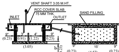
SECTION ON SEPTIC TANK & DISP-TRENCH
