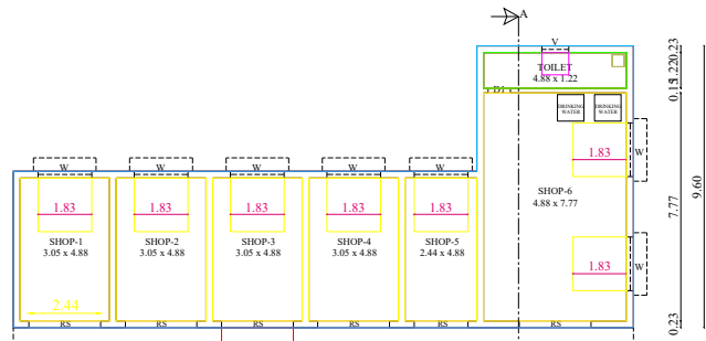
PROPOSED GROUND FLOOR SHOP PLAN
