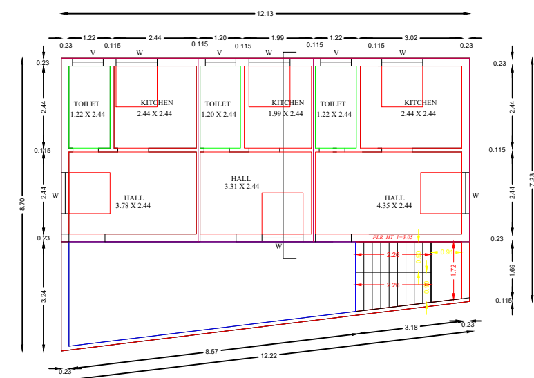
2 FLOOR
