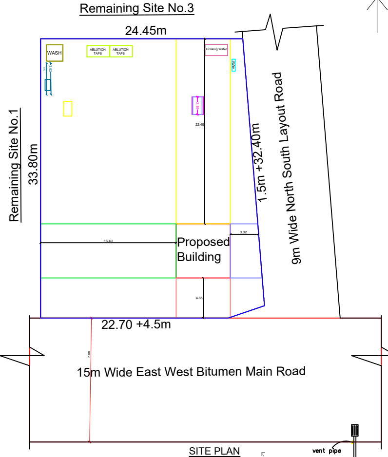
SITE PLAN
