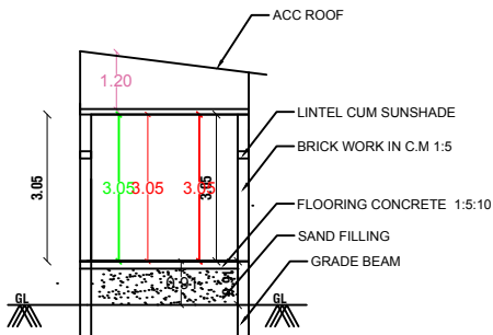
SECTION-AB
