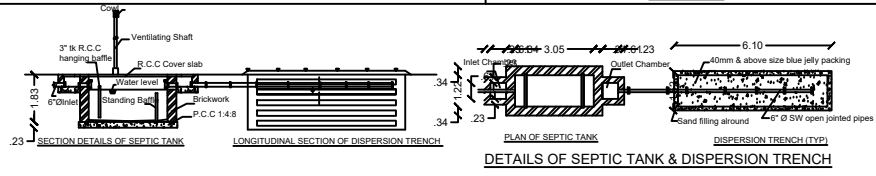
DETAILS OF SEPTIC TANK & DISPERSION TRENCH
