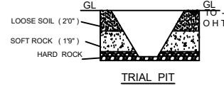
TRIAL PIT
