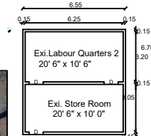
PLAN (North Facing)
