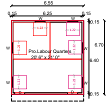
GROUND FLOOR PLAN (East Facing)
