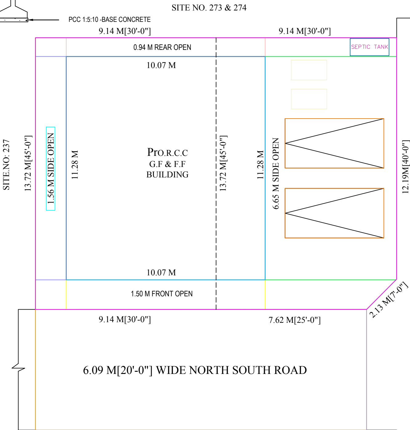
SITE PLAN
