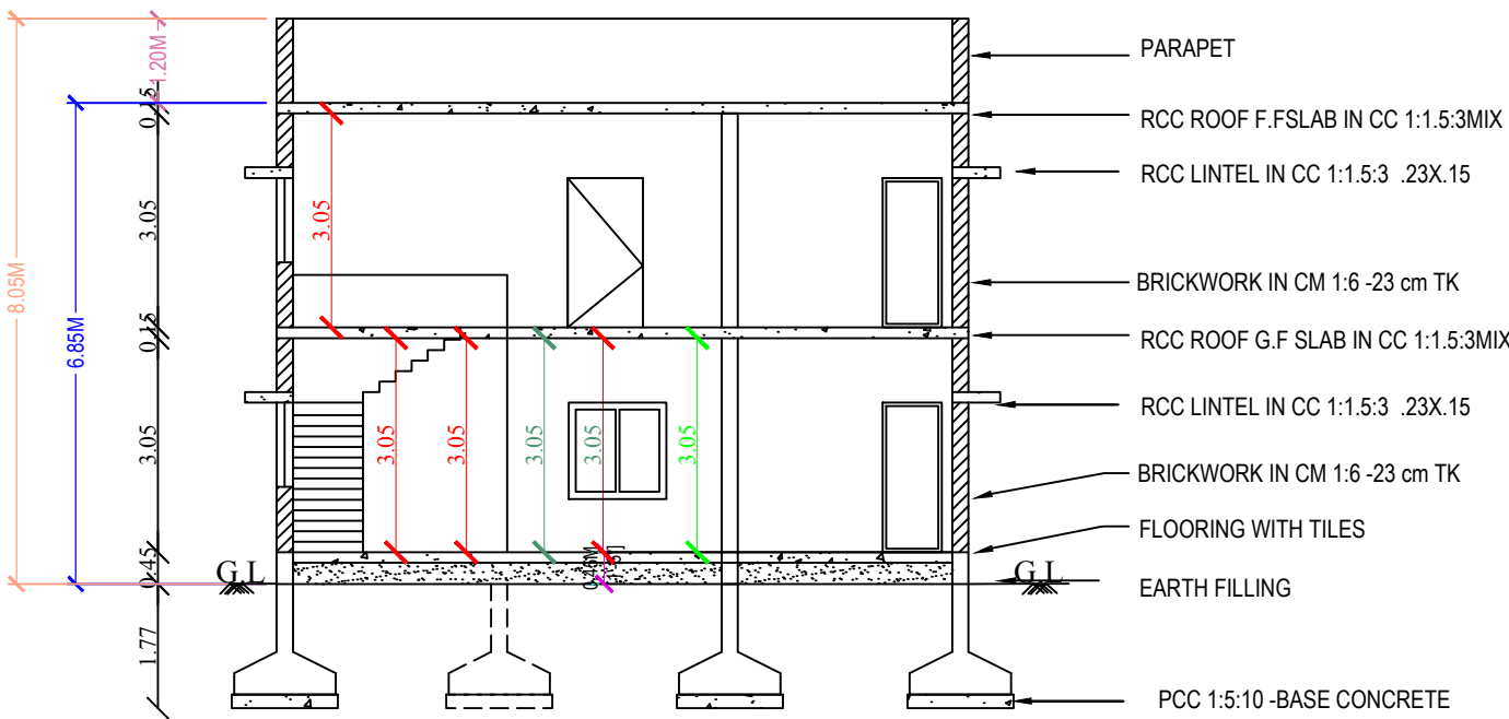
SECTION AA
