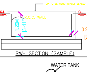
WATER TANK DETAIL
