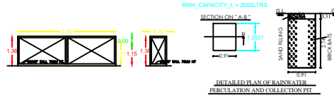
DETAILED PLAN OF RAINWATER PERCOLATION AND COLLECTION PIT
