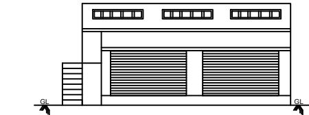
FRONT ELEVATION FACING NORTH
