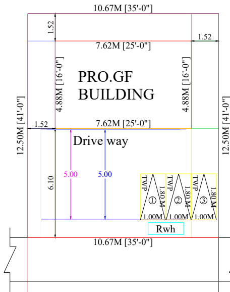
SITE PLAN(NTS)
