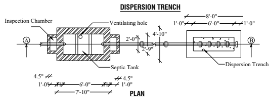
PLAN
