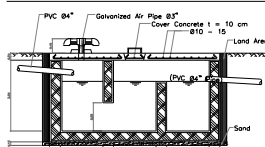
SEPTIC TANK SECTION
