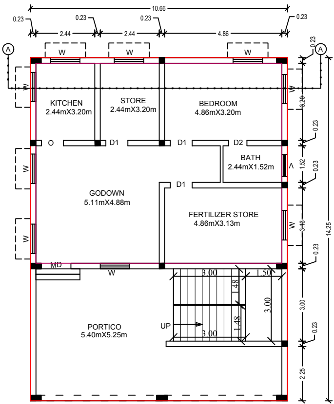
FARM HOUSE FLOOR PLAN
