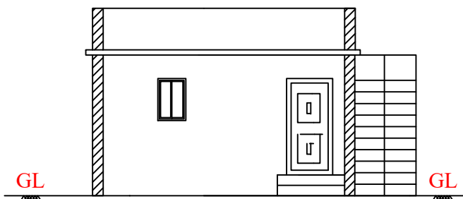
ELEVATION ON EAST FACE
