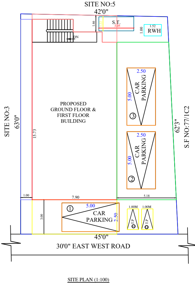
SITE PLAN (1:100)
