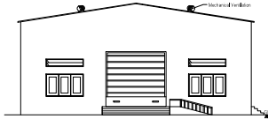
WEST ELEVATION
