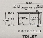
PROPOSED FIRST FLOOR PLAN
