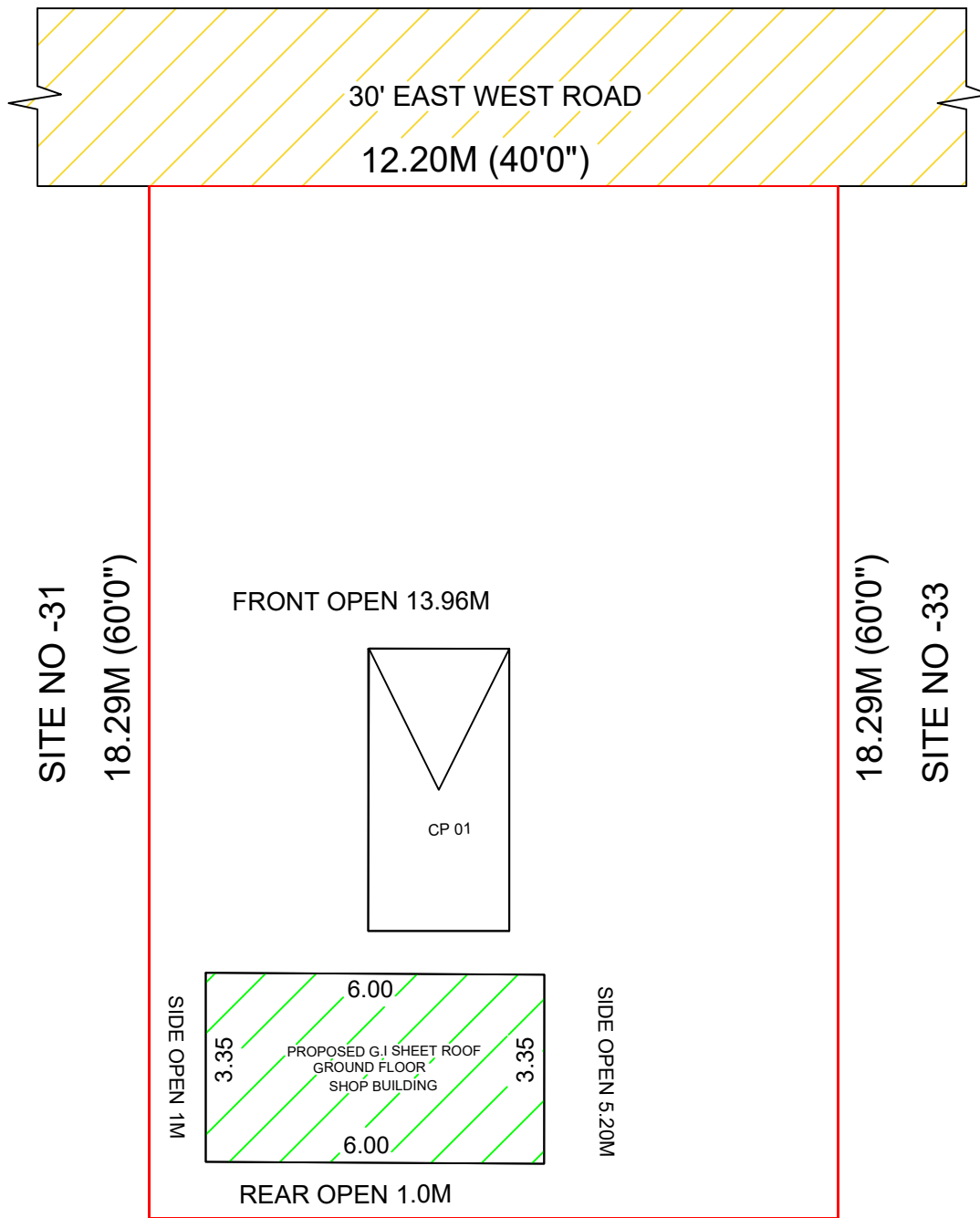
SITE PLAN SCALE-1:200 SHEET-2
