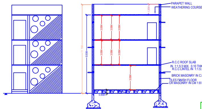
ELEVATION ON NORTH
