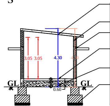
SECTION ON A-B
