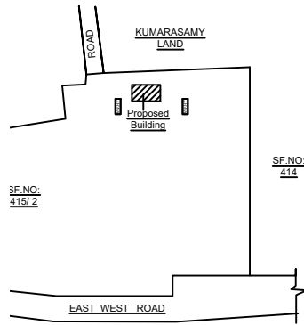
SITE PLAN ( SCALE 1:200 )
