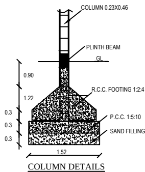
COLUMN DETAILS
