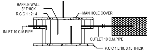
SEPTIC TANK & TRENCH
