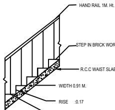
STAIR DETAIL
