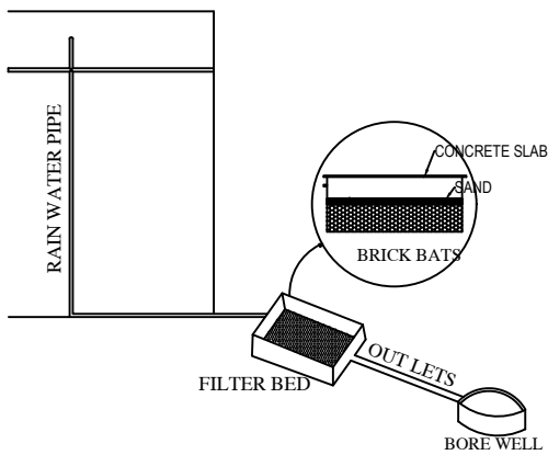
RAIN WATER HARVESTING TANK
