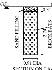
SECTION ON "A-A"
