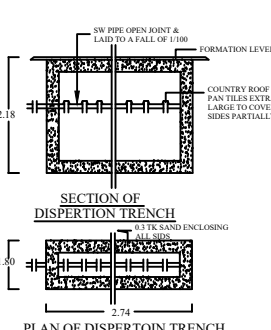
DISPERSION TRENCH
