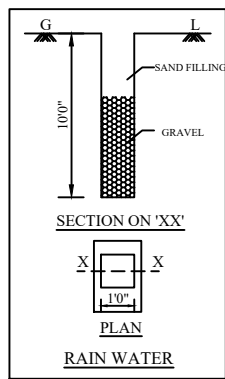
RAINWATER HARVESTING
