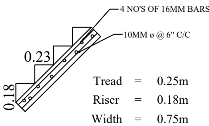
STAIRCASE DETAILS
