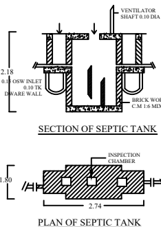
SEPTIC TANK
