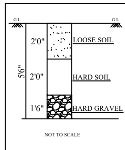
TRIAL PIT
