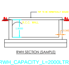
RW_SECTION (SAMPLE)
