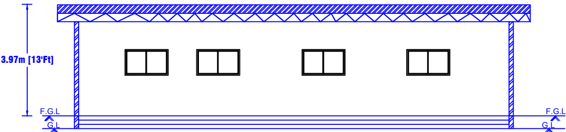
FRONT NORTH ELEVATION
