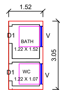
TOILET BLOCK PLAN
