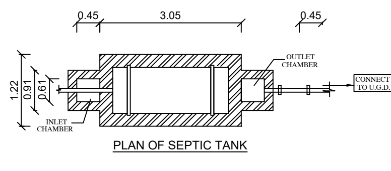
DETAILS OF SEPTIC TANK ( N.T.S. )
