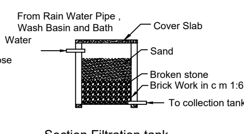
Section Filtration tank
