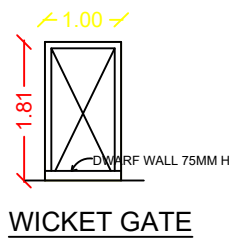
WICKET GATE
