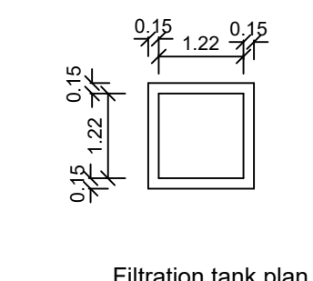
Filtration tank plan
