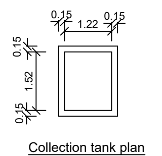
Collection tank plan
