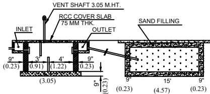
SECTION ON SEPTIC TANK & DISP-TRENCH
