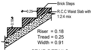
STAIR DETAILS (NOT TO SCALE)
