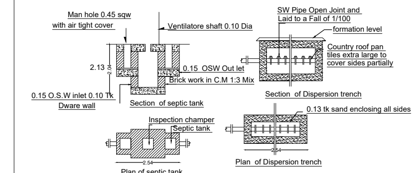
DETAILED DRAWING FOR SEPTIC TANK WITH DISPERSION TRENCH 225 GALONS CAPACITY OF 1000 LITRES
