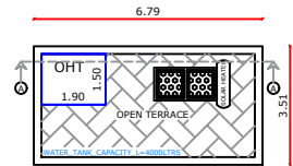
PROPOSED TERRACE FLOOR PLAN
