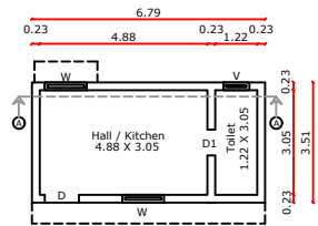
PROPOSED GROUND FLOOR PLAN
