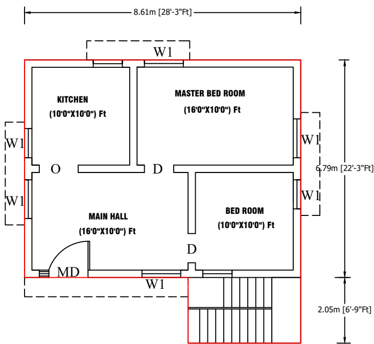
GROUND FLOOR PLAN ON NORTH FACE
