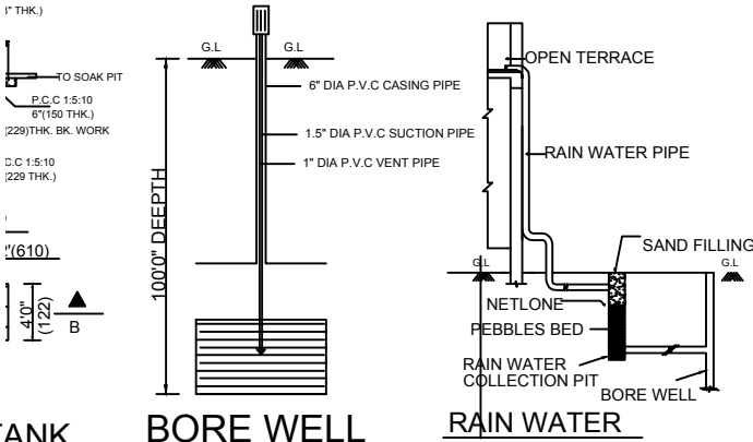
BORE WELL
