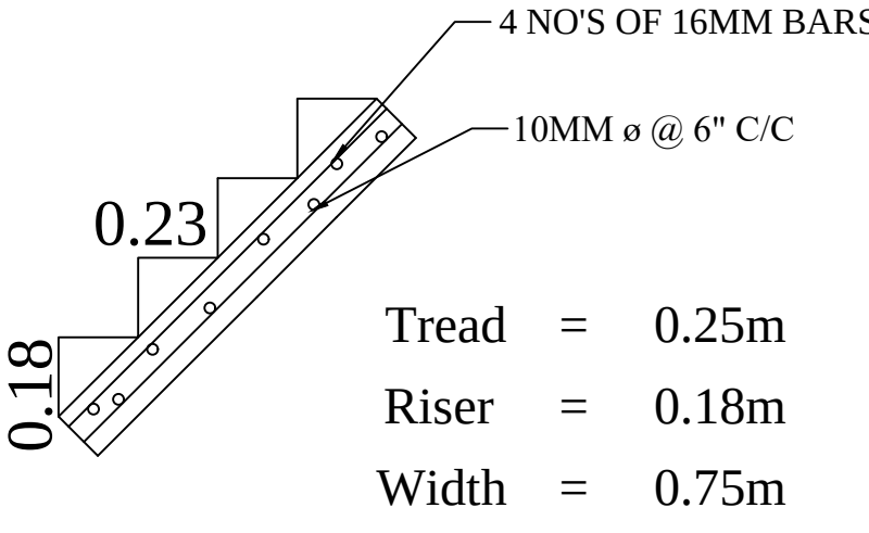
STAIRCASE DETAILS
