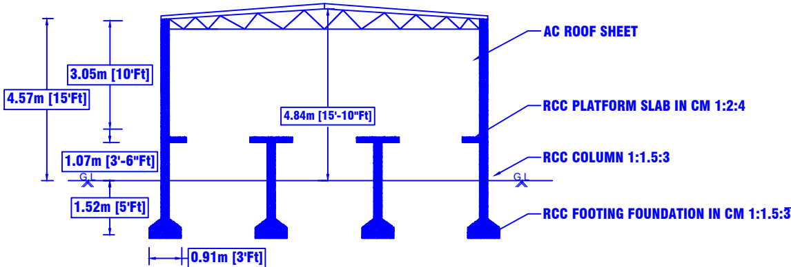
SECTION ON-AA
