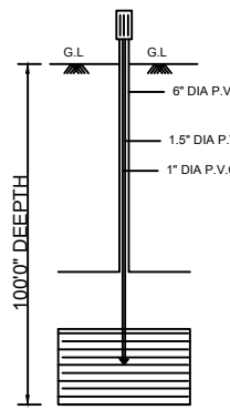
BORE WELL
