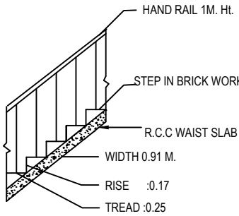
STAIR DETAIL
