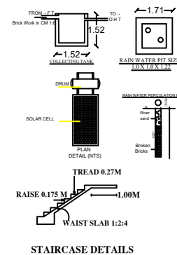
STAIRCASE DETAILS
