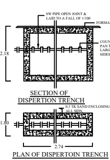
DISPERSION TRENCH
