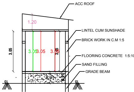
SECTION-AB
