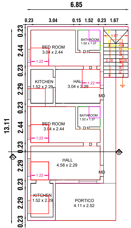
PRO. GROUND FLOOR PLAN.
