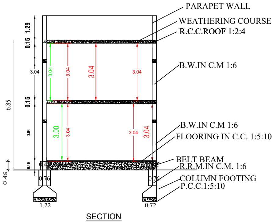
SECTION
