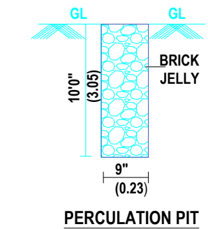
PERCOLATION PIT
