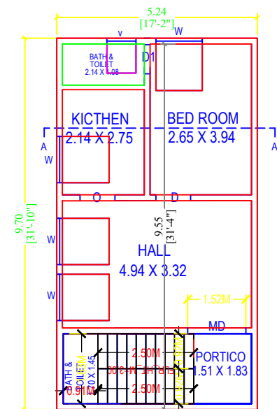
PRO.GROUND FLOOR
